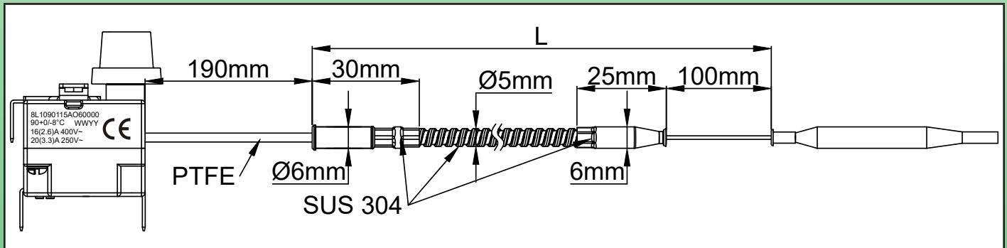
8A Thermostat, SPDT or SPNC reset (not fail safe)
