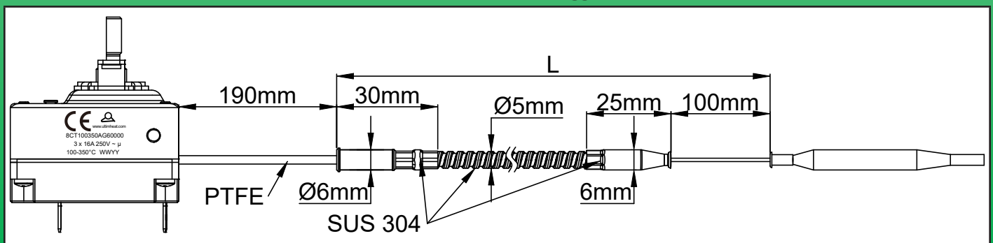
8C Thermostat, 3PNC control, staggered contacts
