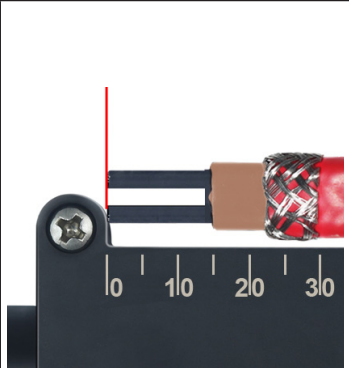
4: Graduated scale in cm, engraved, with mechanical stop at 0 cm , to ease the stripping length measurement.
