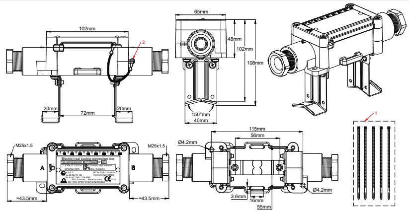
Example of mounting at distance of the pipe with the long legs stainless steel bracket (Mounting option 5)
