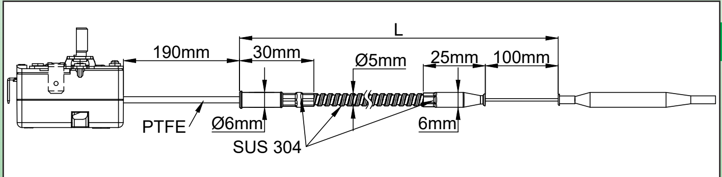
8L Thermostat, SPNC reset, fail safe
